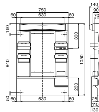
MK-751THL
